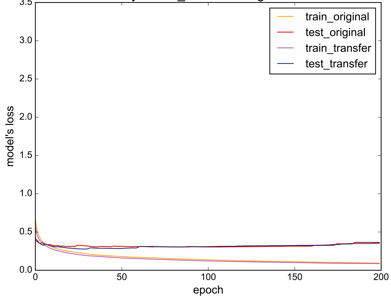
Source: synthetic_control - Target: ECG5000
