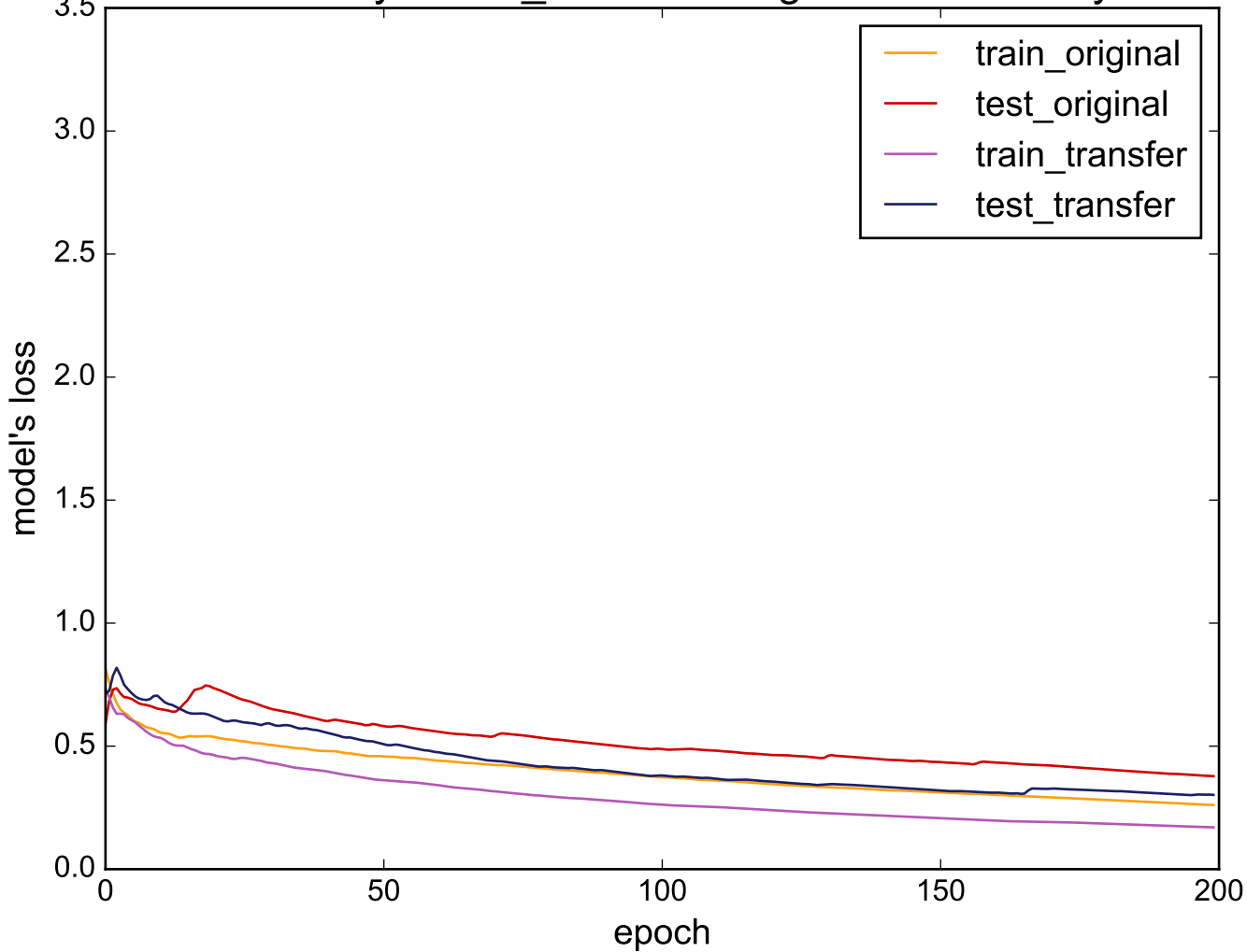
Source: synthetic_control - Target: ECGFiveDays
