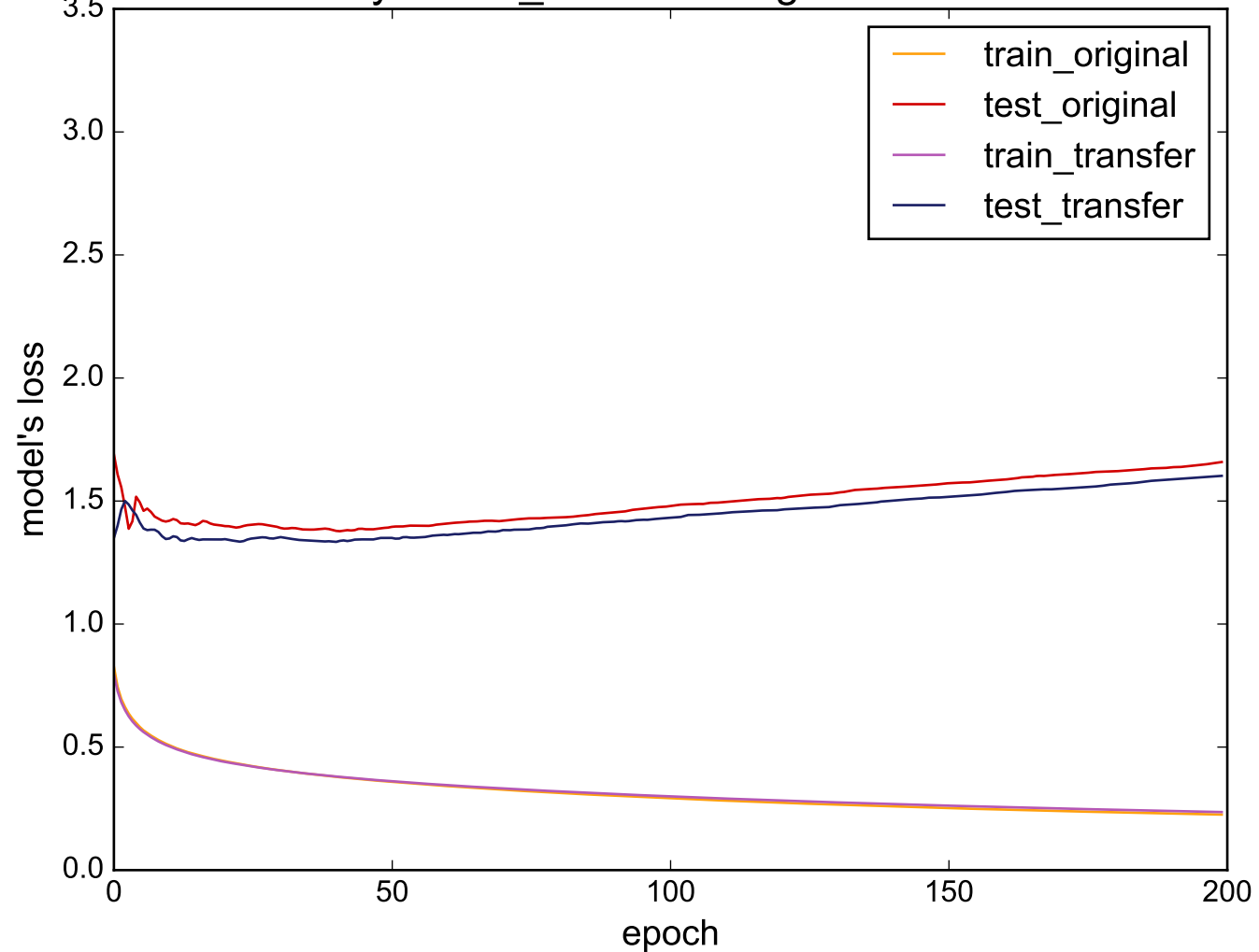
Source: synthetic_control - Target: ElectricDevices
