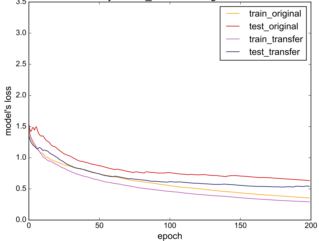
Source: synthetic_control - Target: FaceFour
