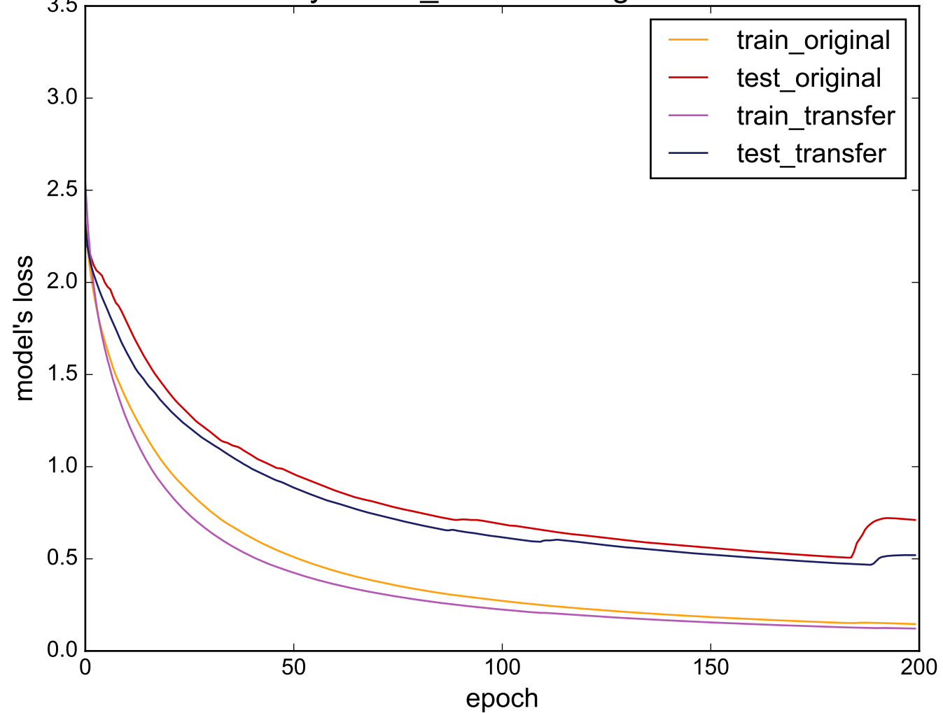
Source: synthetic_control - Target: FacesUCR
