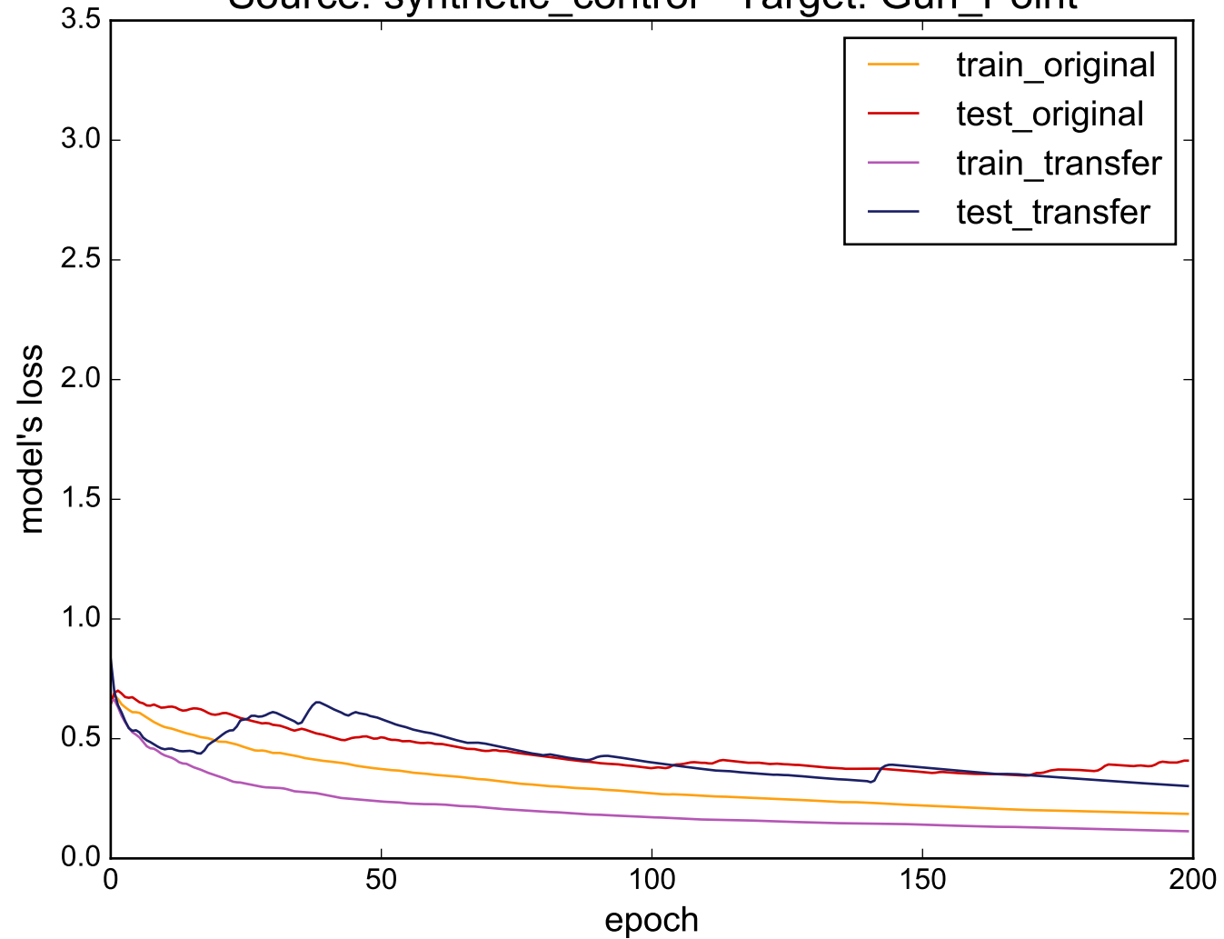
Source: synthetic_control - Target: Gun_Point
