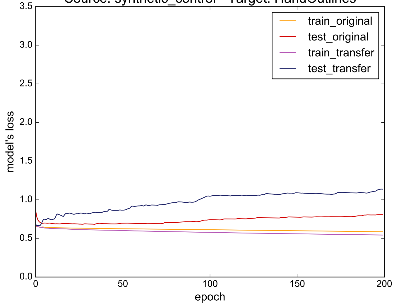
Source: synthetic_control - Target: HandOutlines
