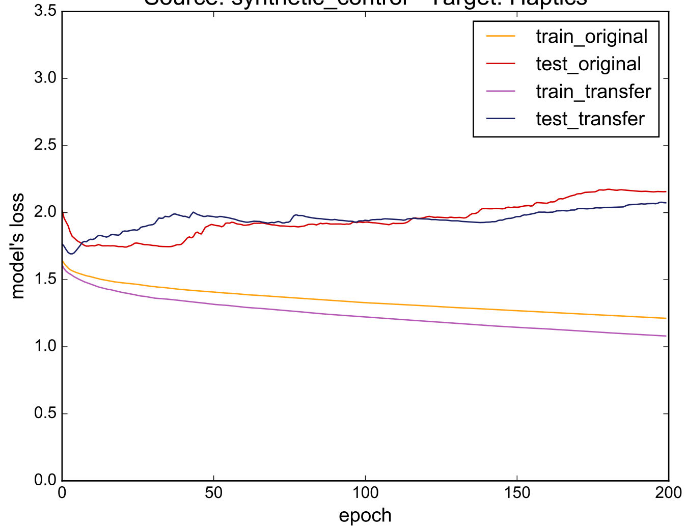
Source: synthetic_control - Target: Haptics
