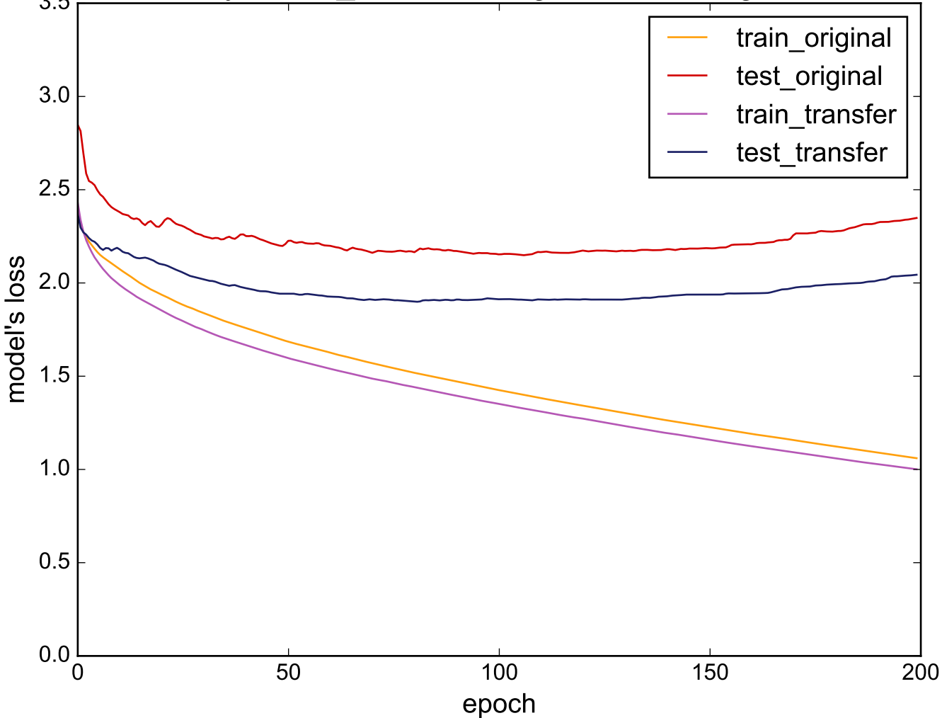
Source: synthetic_control - Target: InsectWingbeatSound
