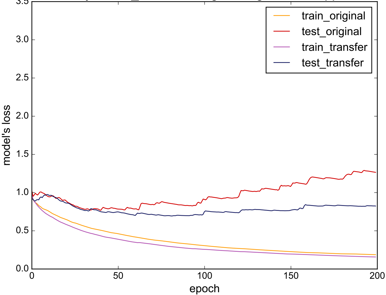
Source: synthetic_control - Target: LargeKitchenAppliances
