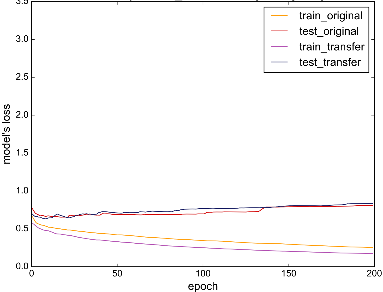
Source: synthetic_control - Target: Lighting2
