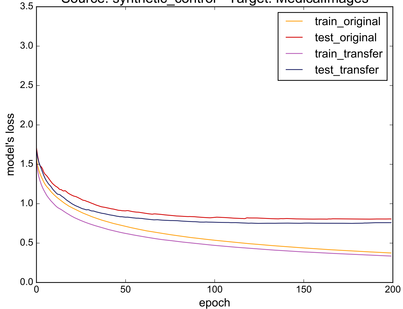
Source: synthetic_control - Target: MedicalImages
