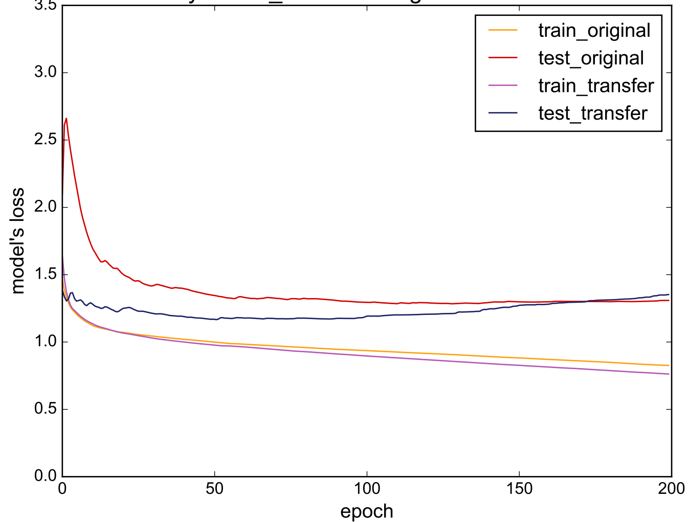
Source: synthetic_control - Target: MiddlePhalanxTW
