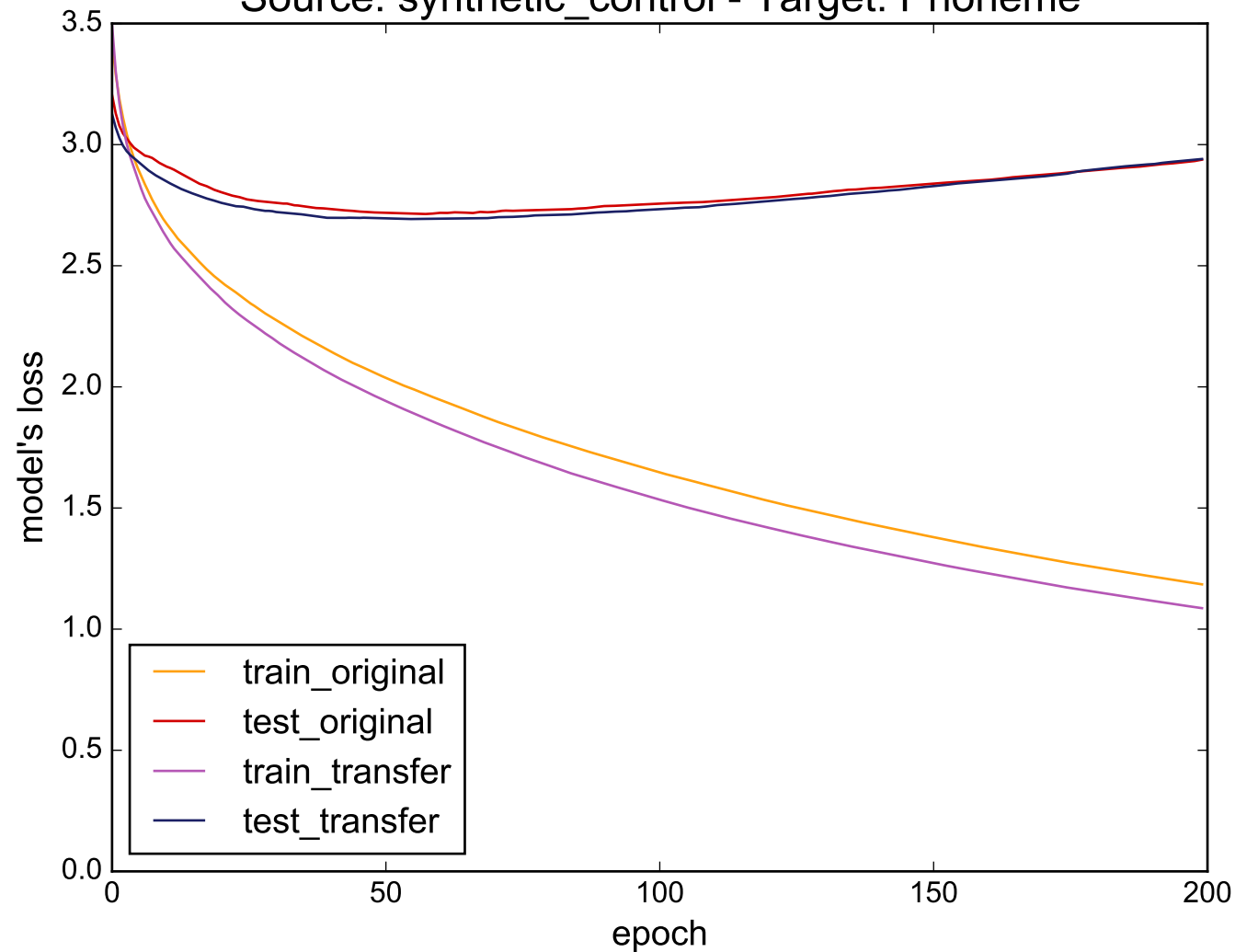
Source: synthetic_control - Target: Phoneme
