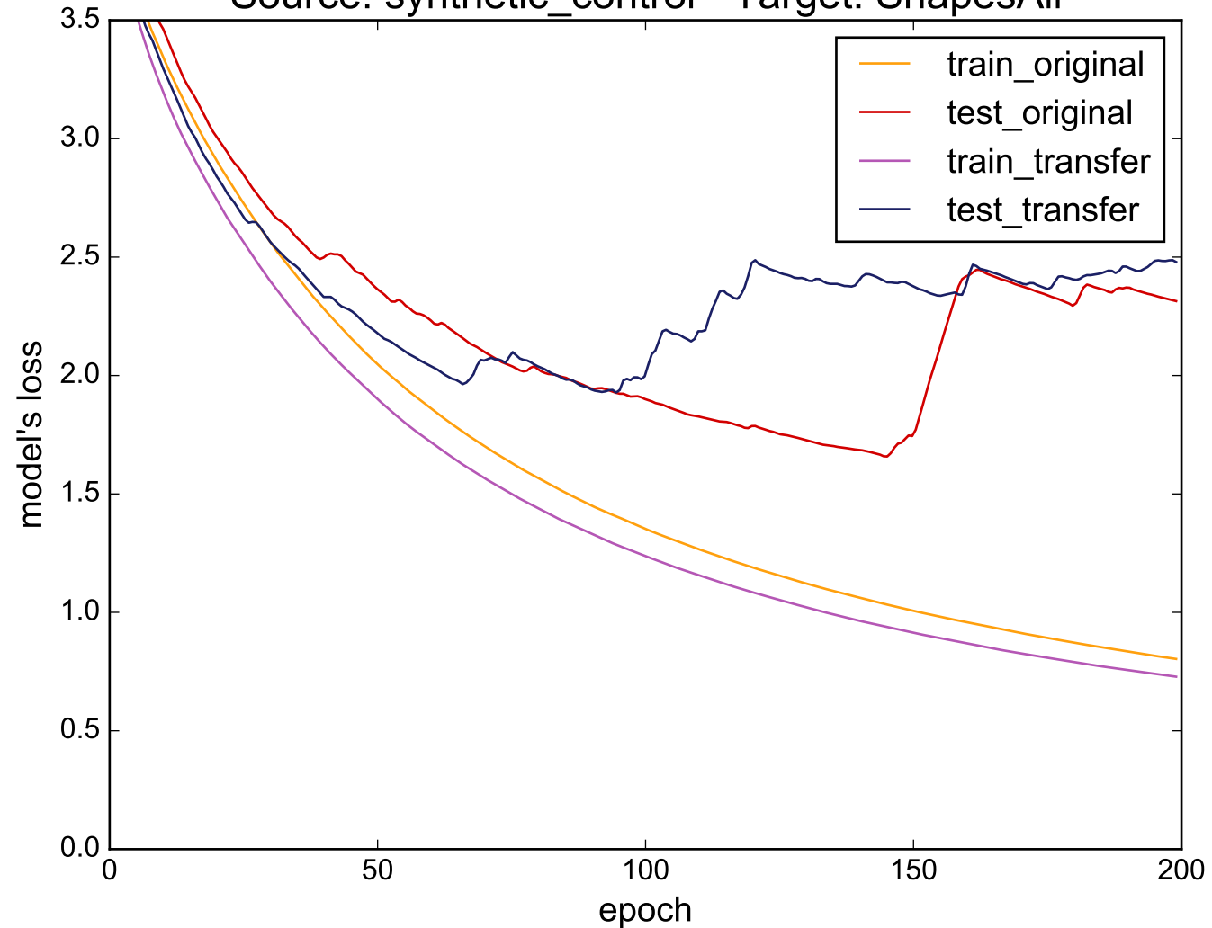
Source: synthetic_control - Target: ShapesAll
