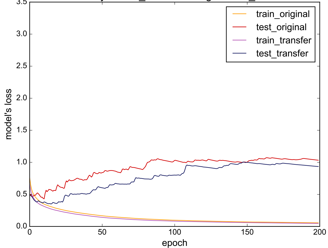
Source: synthetic_control - Target: Two_Patterns
