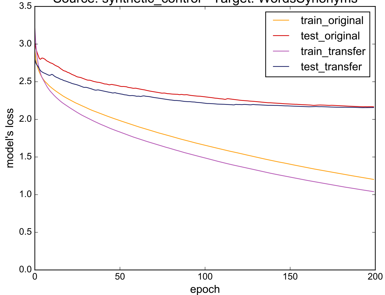
Source: synthetic_control - Target: WordsSynonyms
