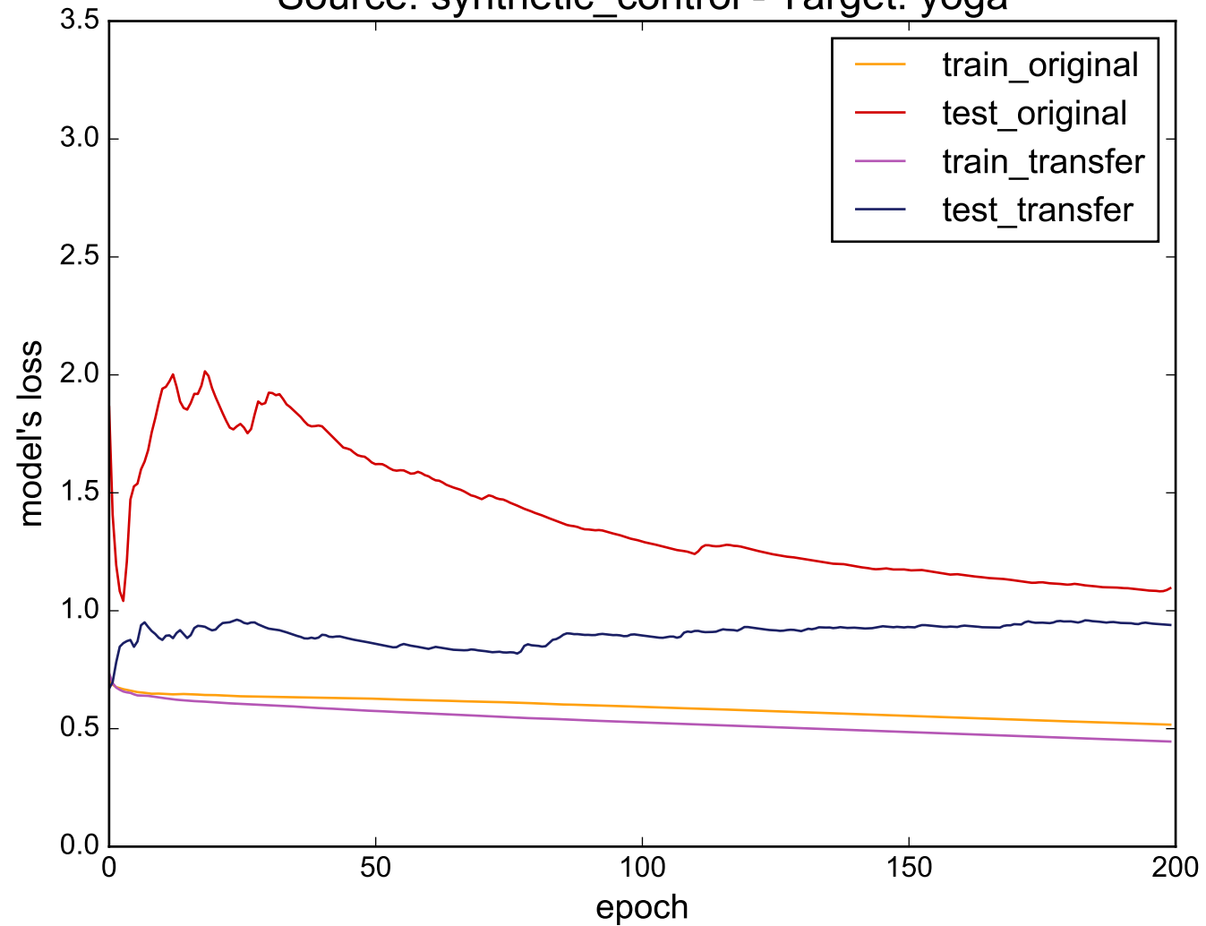
Source: synthetic_control - Target: yoga
