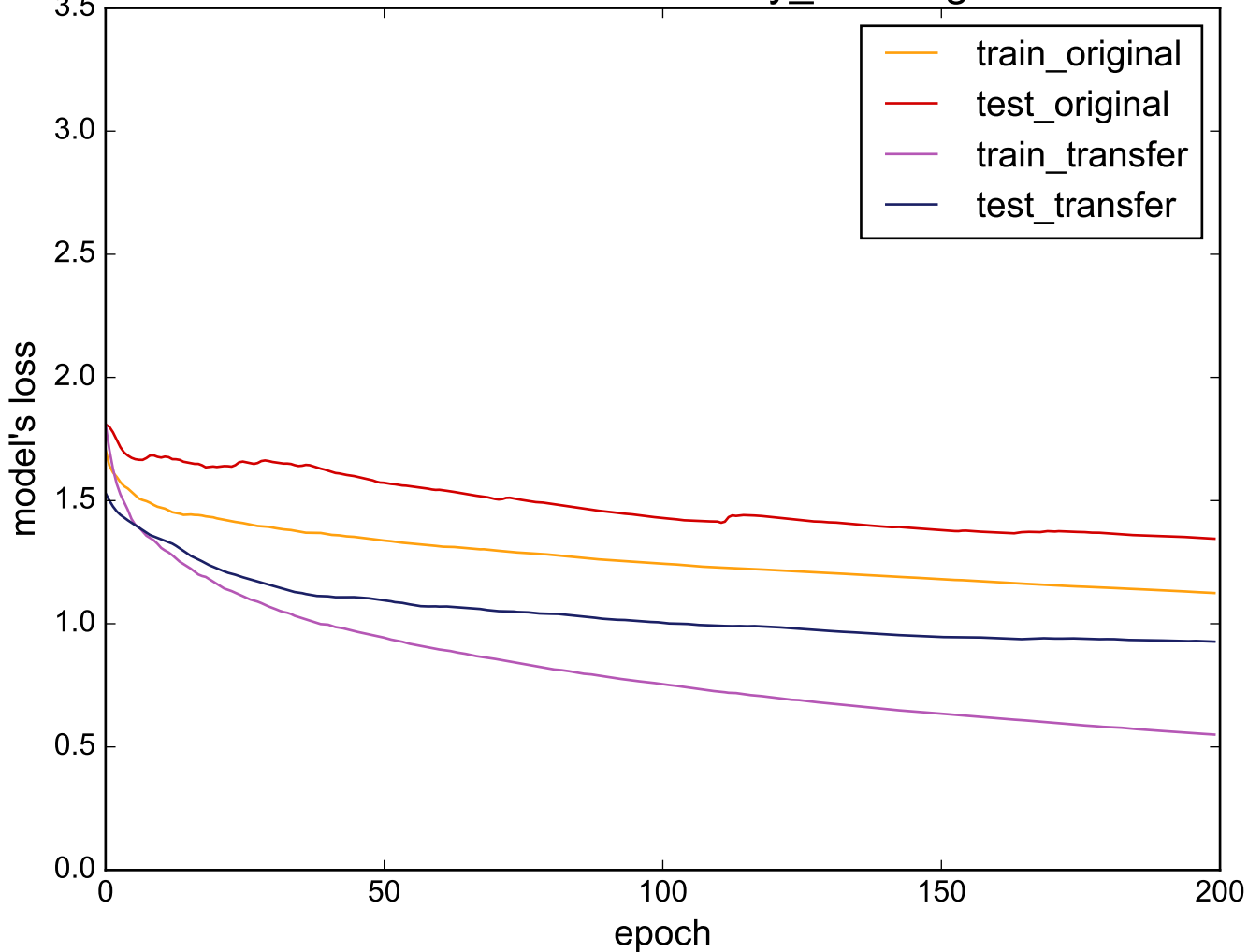
Source: uWaveGestureLibrary_X - Target: Beef
