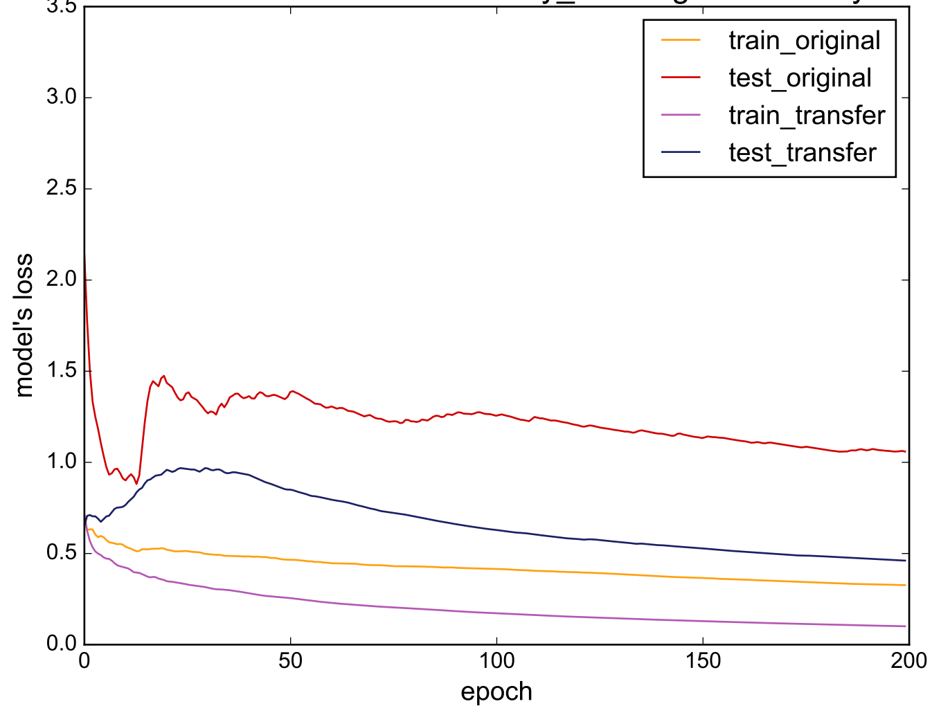
Source: uWaveGestureLibrary_X - Target: BeetleFly
