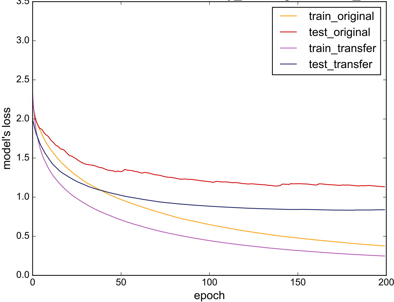
Source: uWaveGestureLibrary_X - Target: Cricket_Y
