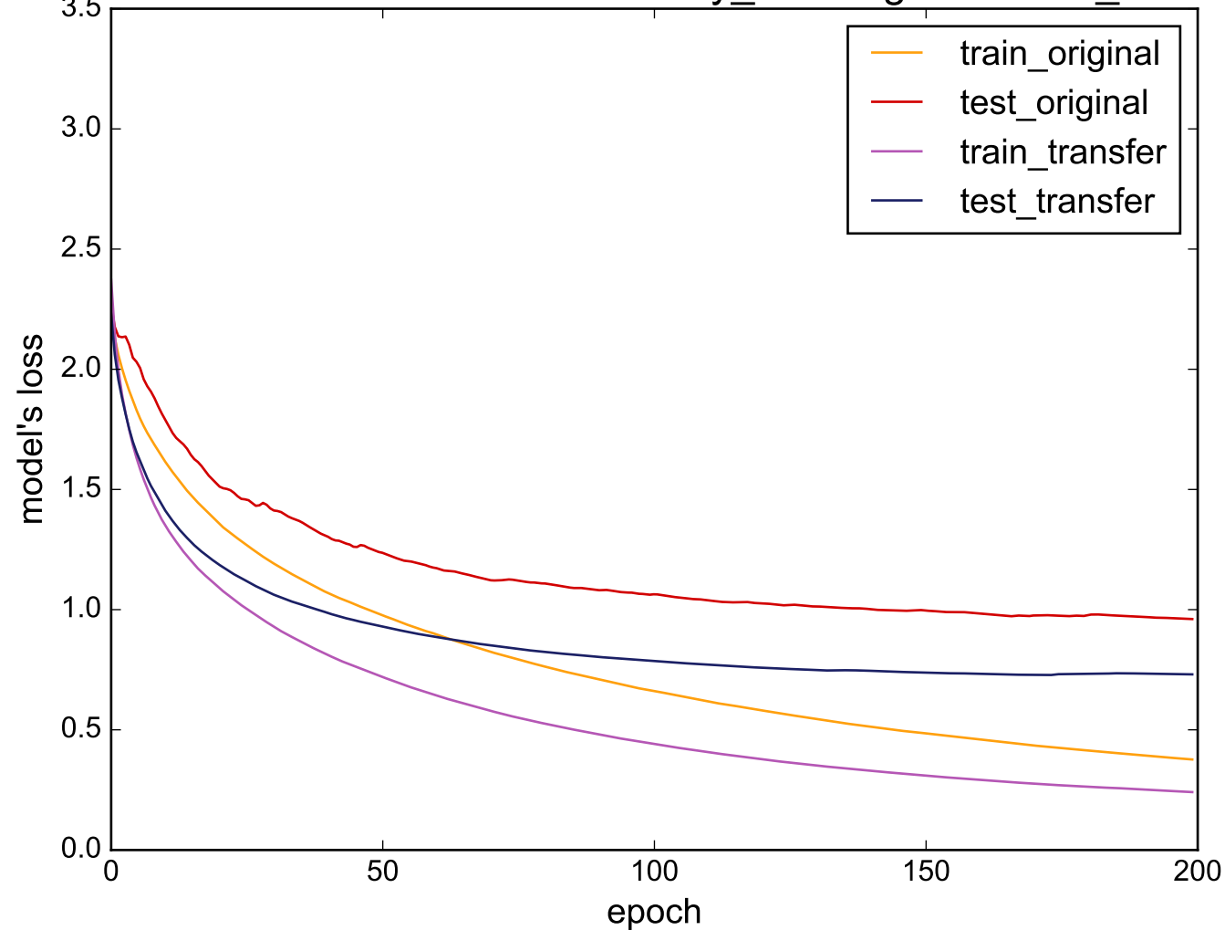
Source: uWaveGestureLibrary_X - Target: Cricket_Z
