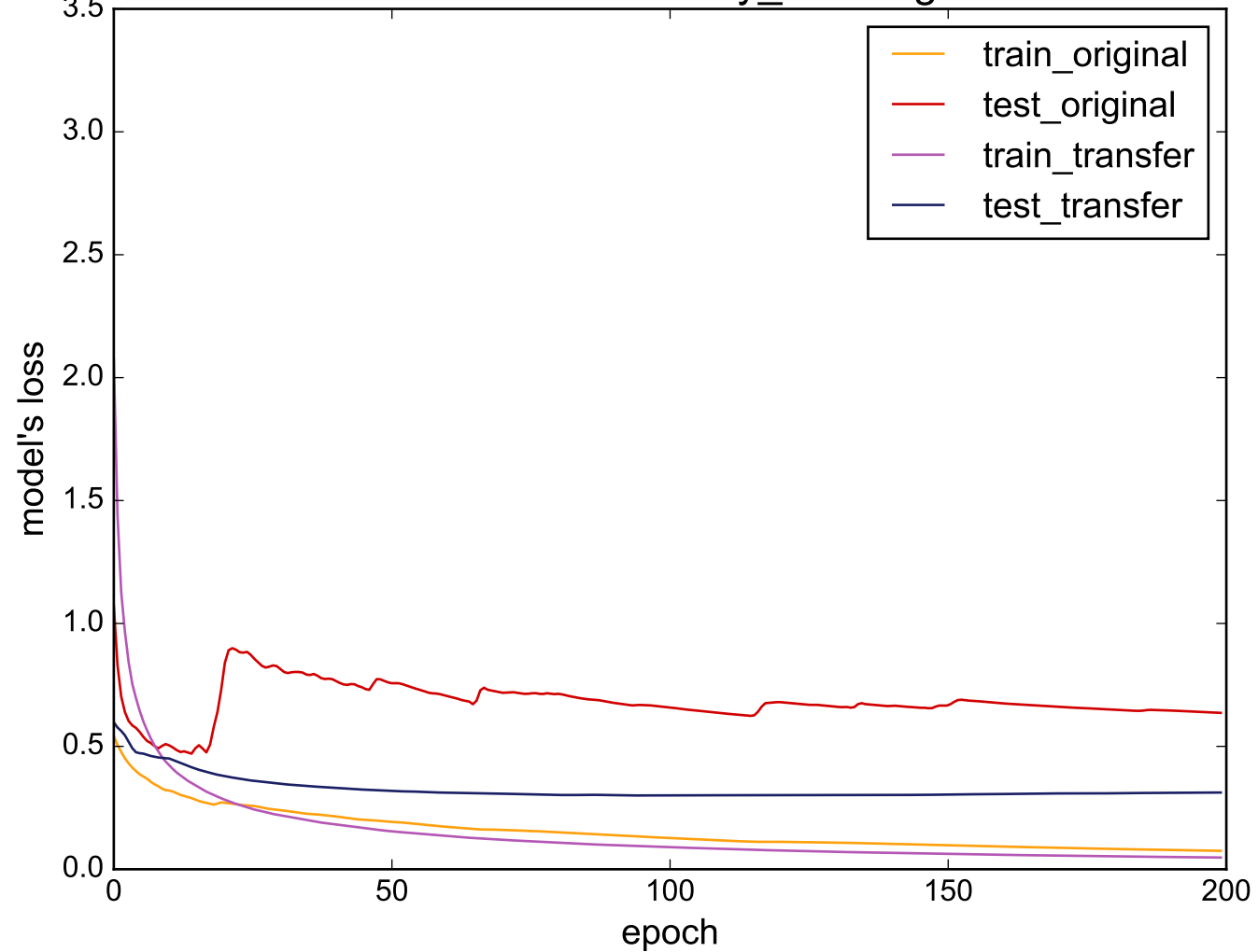
Source: uWaveGestureLibrary_X - Target: ECG200
