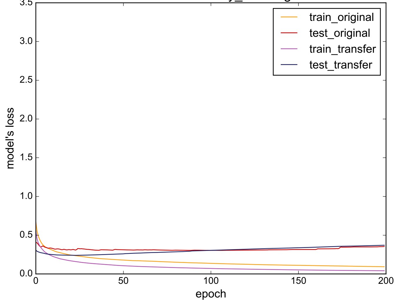
Source: uWaveGestureLibrary_X - Target: ECG5000
