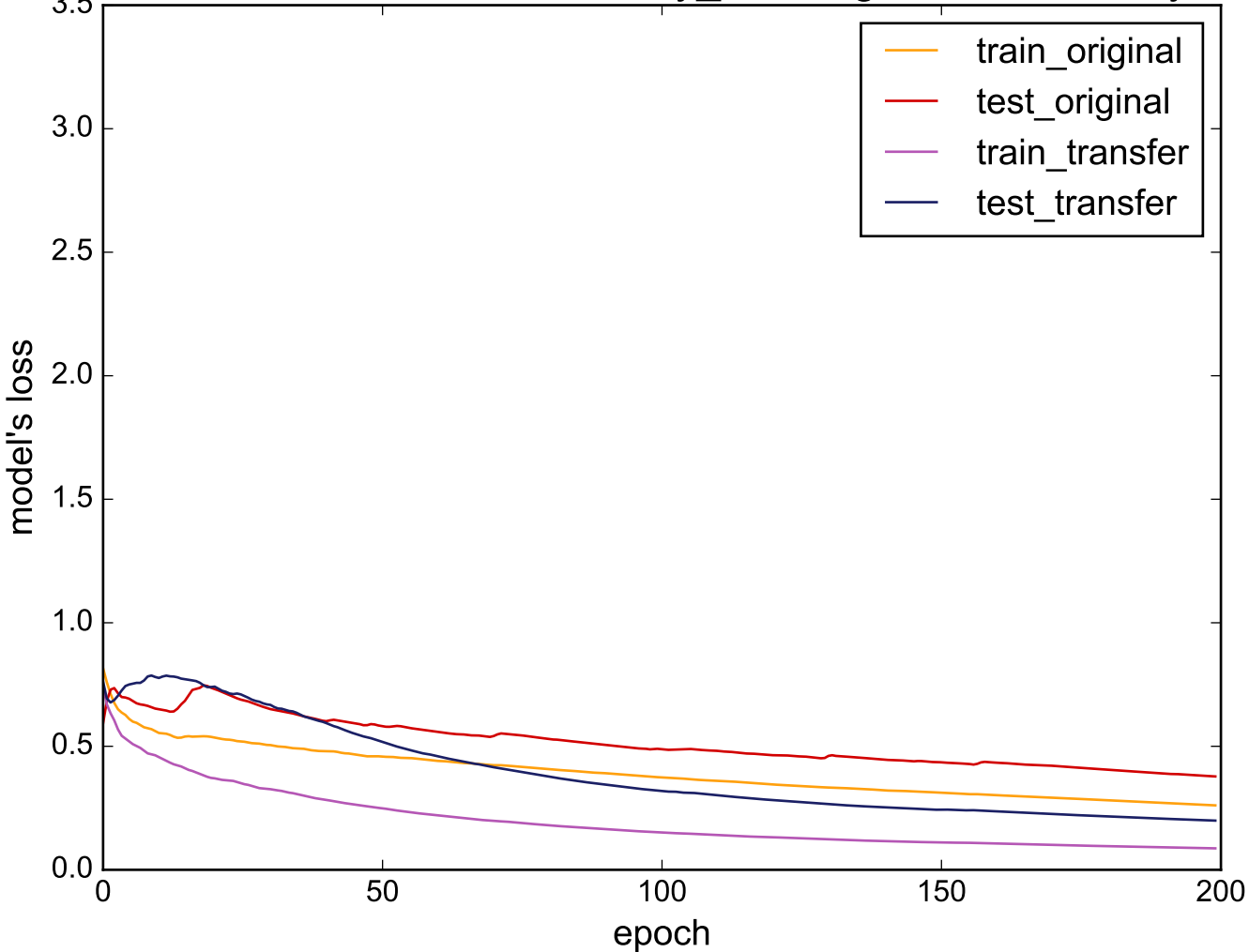
Source: uWaveGestureLibrary_X - Target: ECGFiveDays
