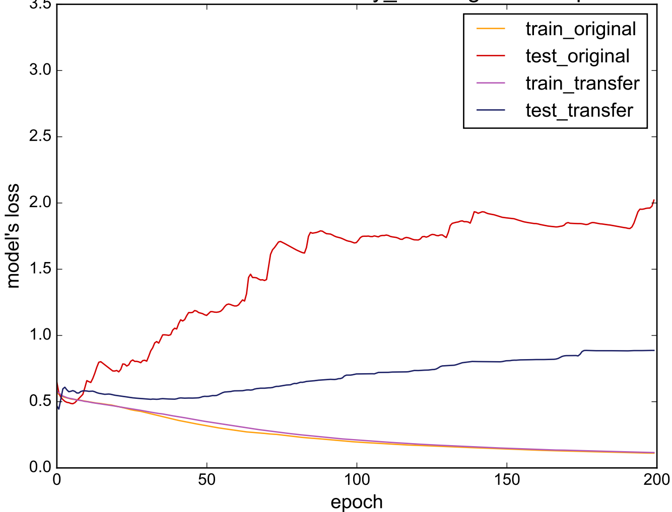
Source: uWaveGestureLibrary_X - Target: Earthquakes
