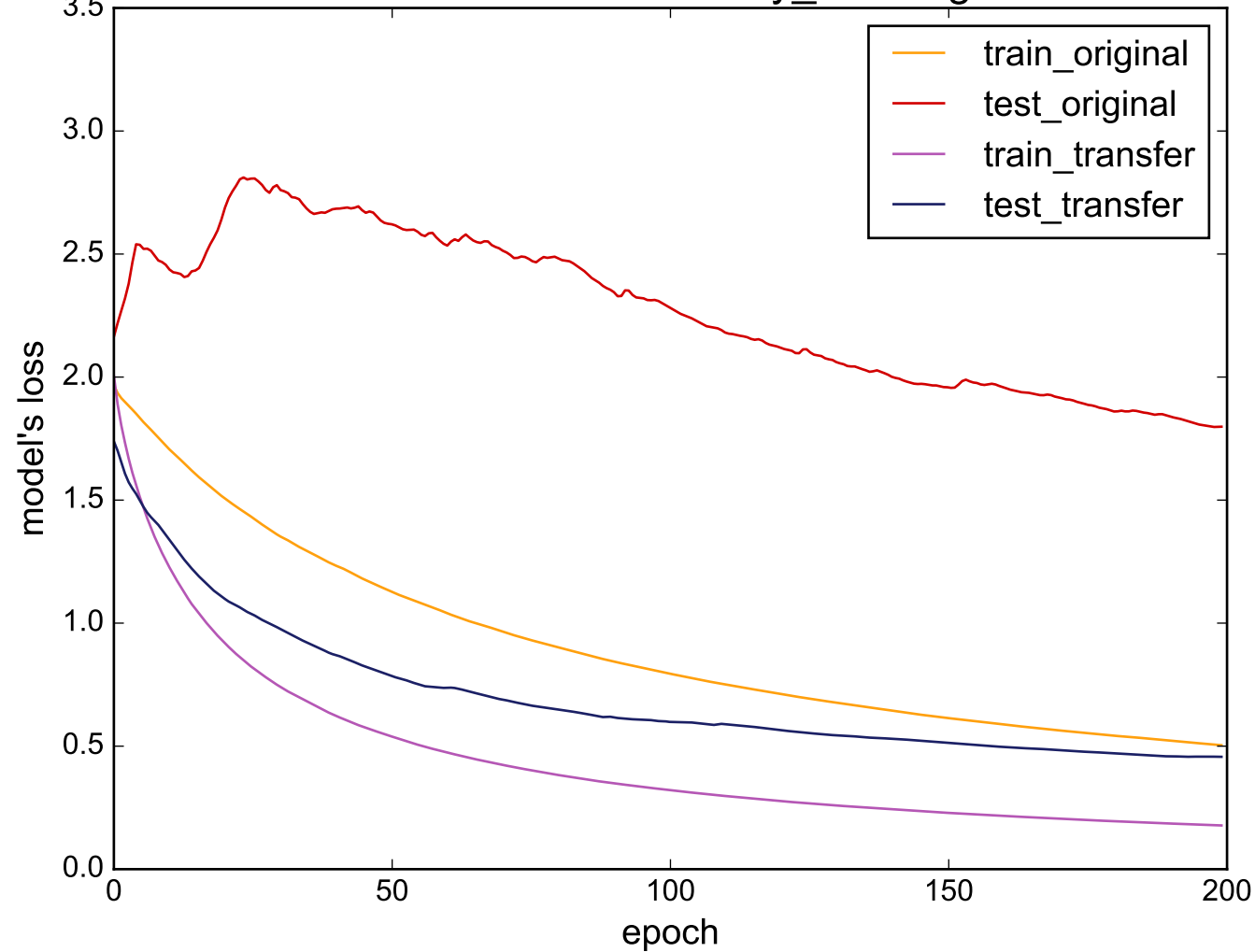
Source: uWaveGestureLibrary_X - Target: FISH
