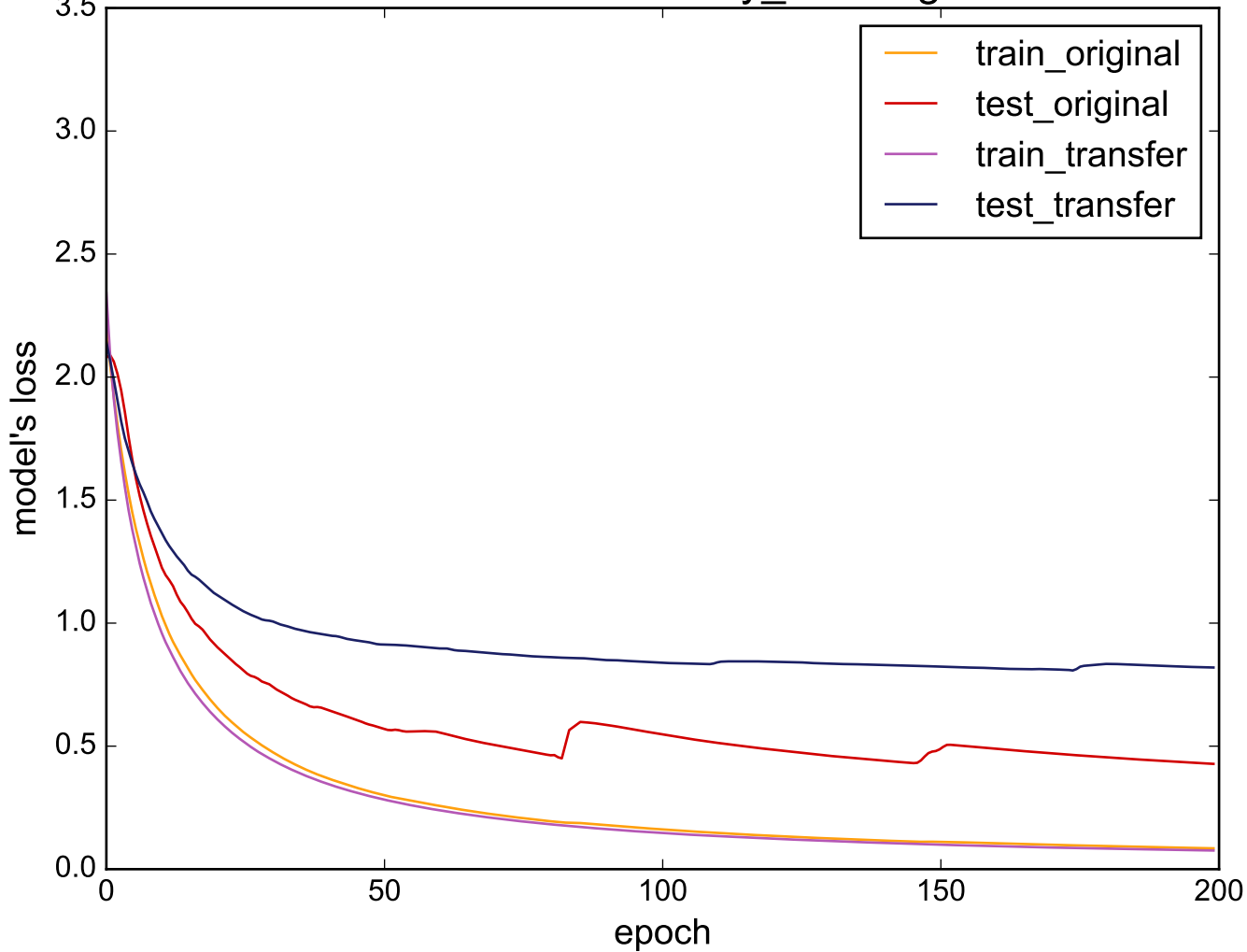
Source: uWaveGestureLibrary_X - Target: FaceAll
