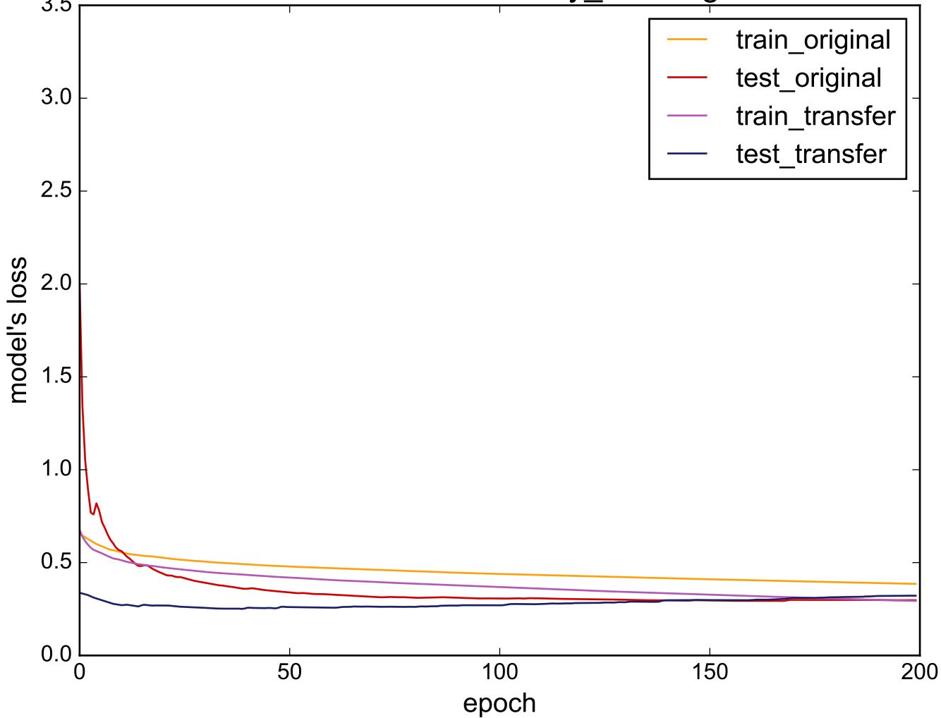
Source: uWaveGestureLibrary_X - Target: FordB
