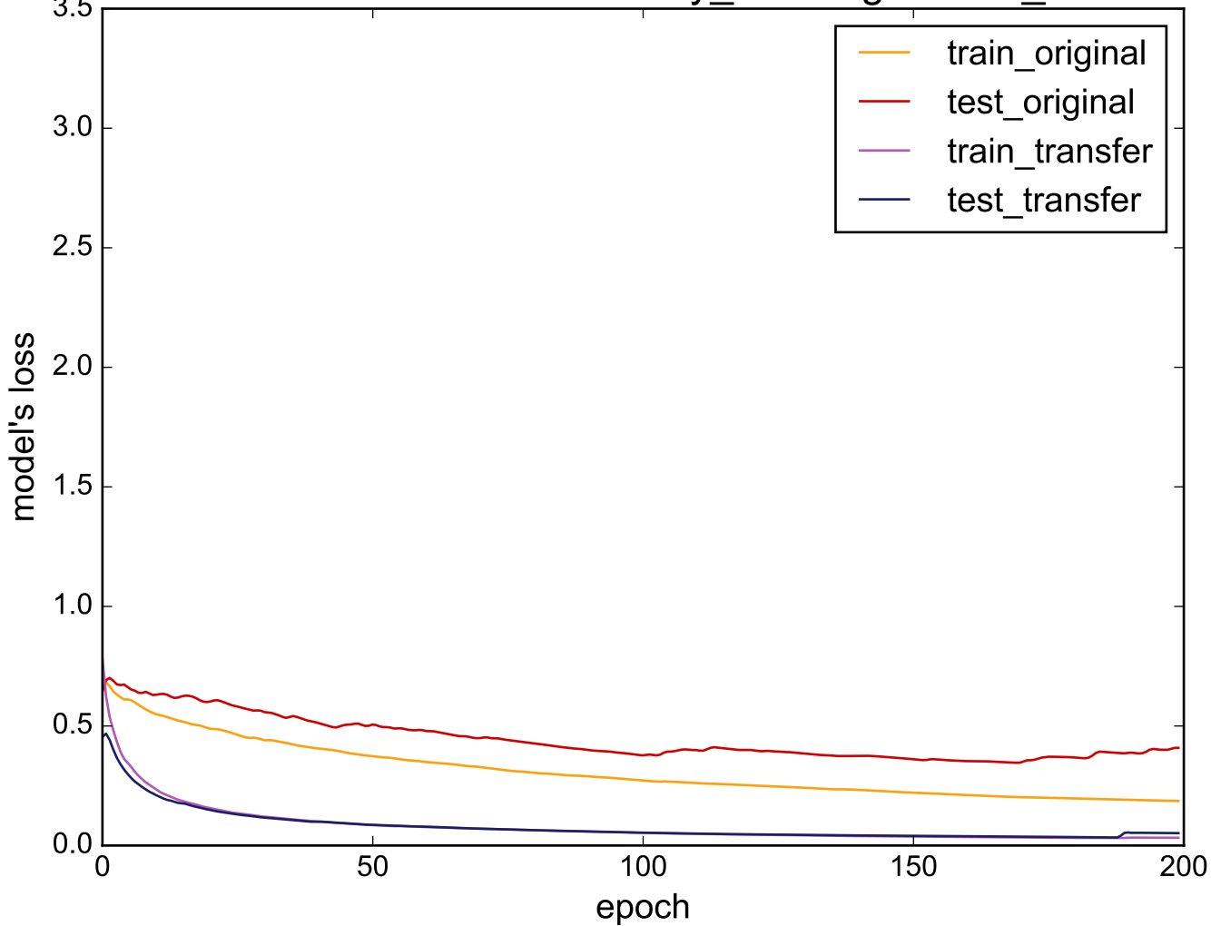
Source: uWaveGestureLibrary_X - Target: Gun_Point
