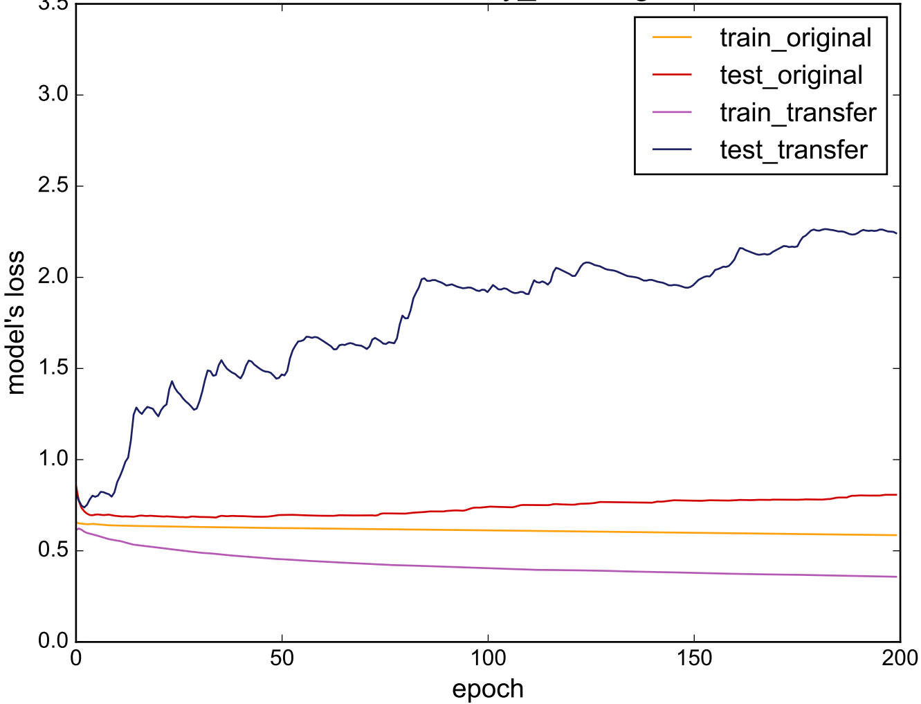
Source: uWaveGestureLibrary_X - Target: HandOutlines
