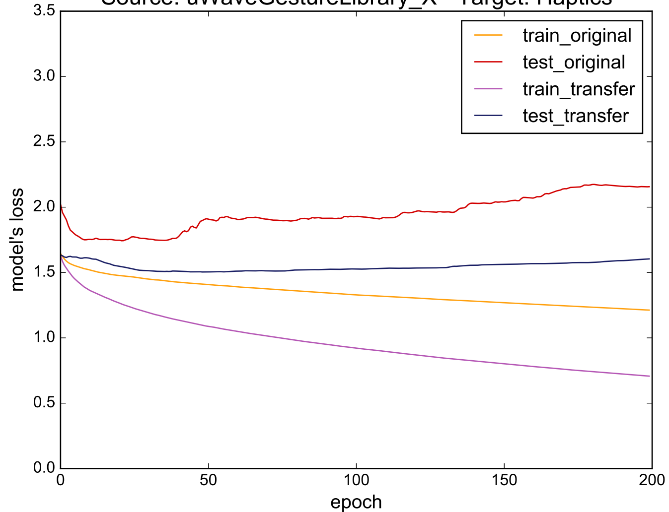
Source: uWaveGestureLibrary_X - Target: Haptics
