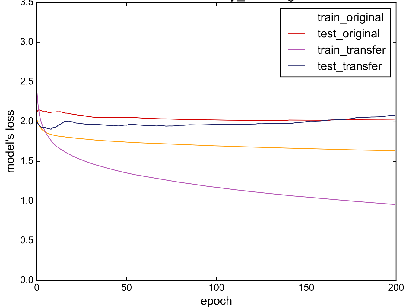
Source: uWaveGestureLibrary_X - Target: InlineSkate
