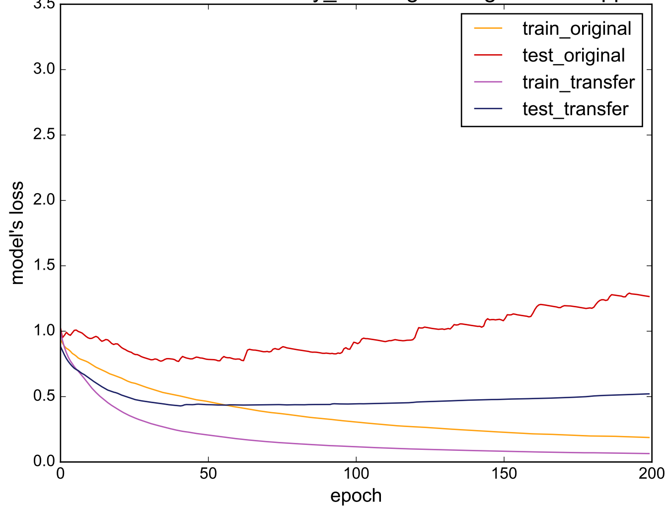
Source: uWaveGestureLibrary_X - Target: LargeKitchenAppliances
