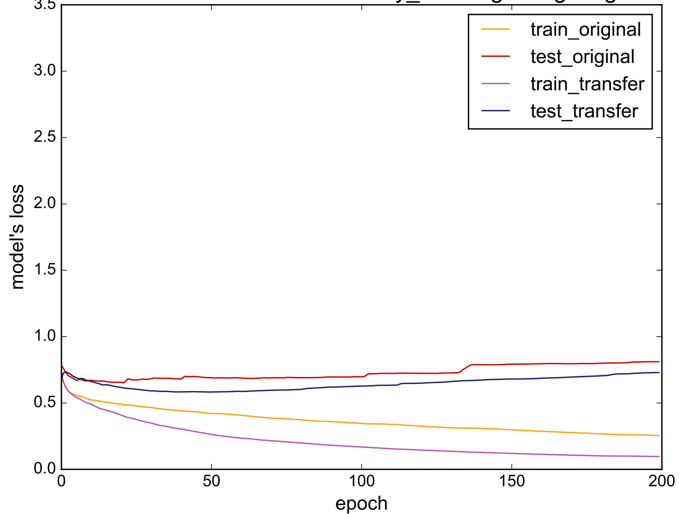
Source: uWaveGestureLibrary_X - Target: Lighting2
