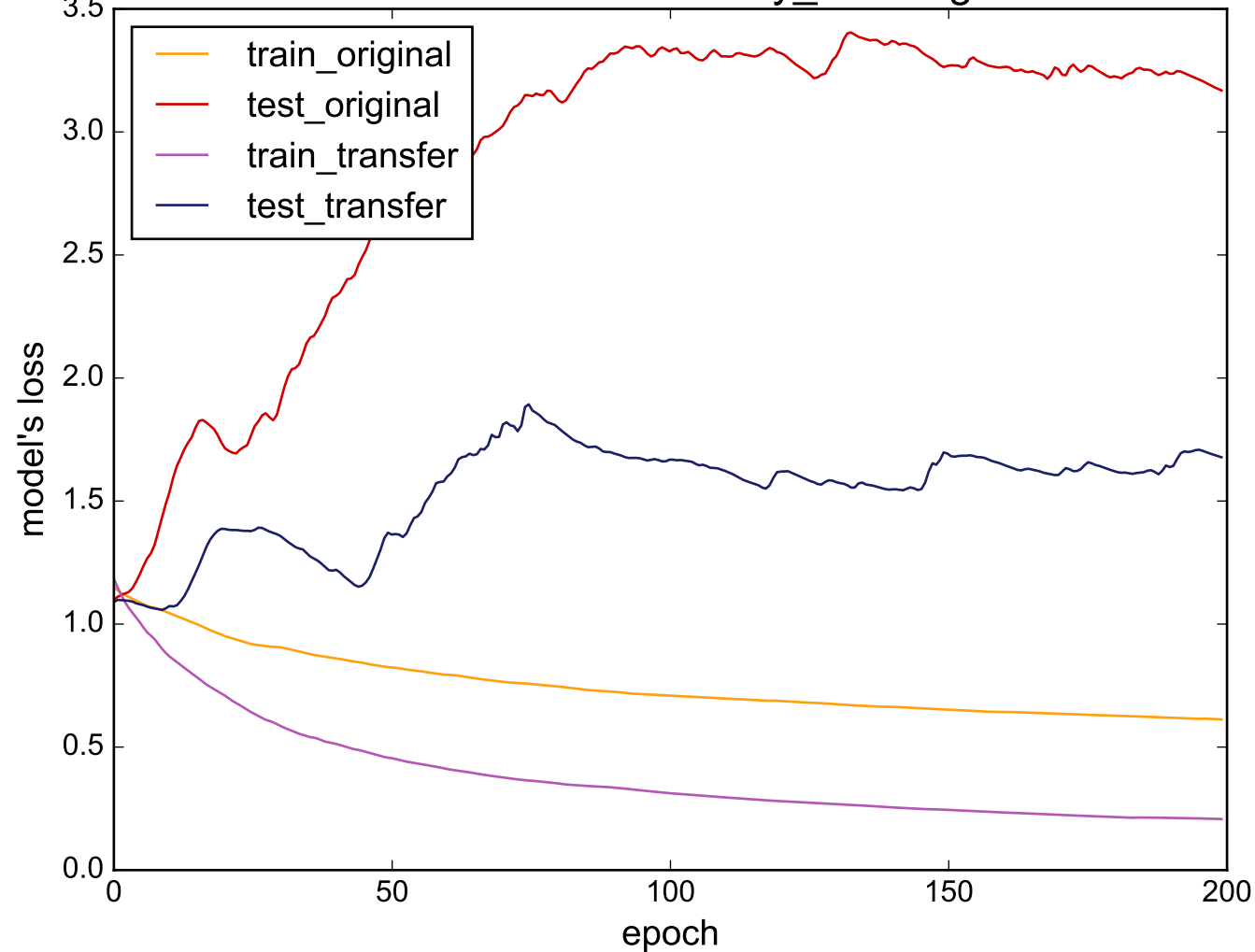
Source: uWaveGestureLibrary_X - Target: Meat
