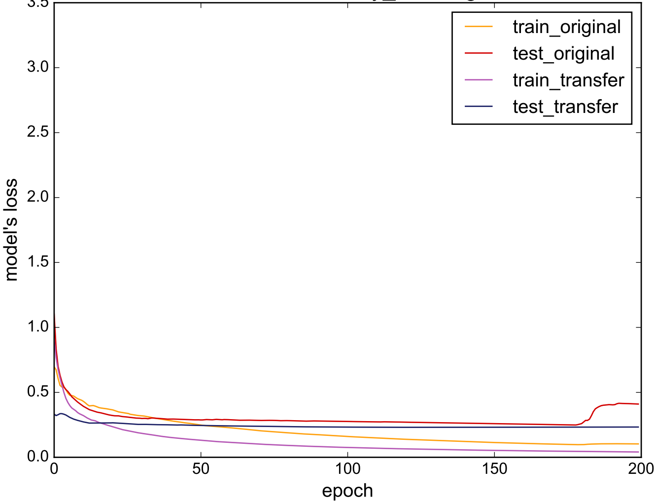
Source: uWaveGestureLibrary_X - Target: MoteStrain
