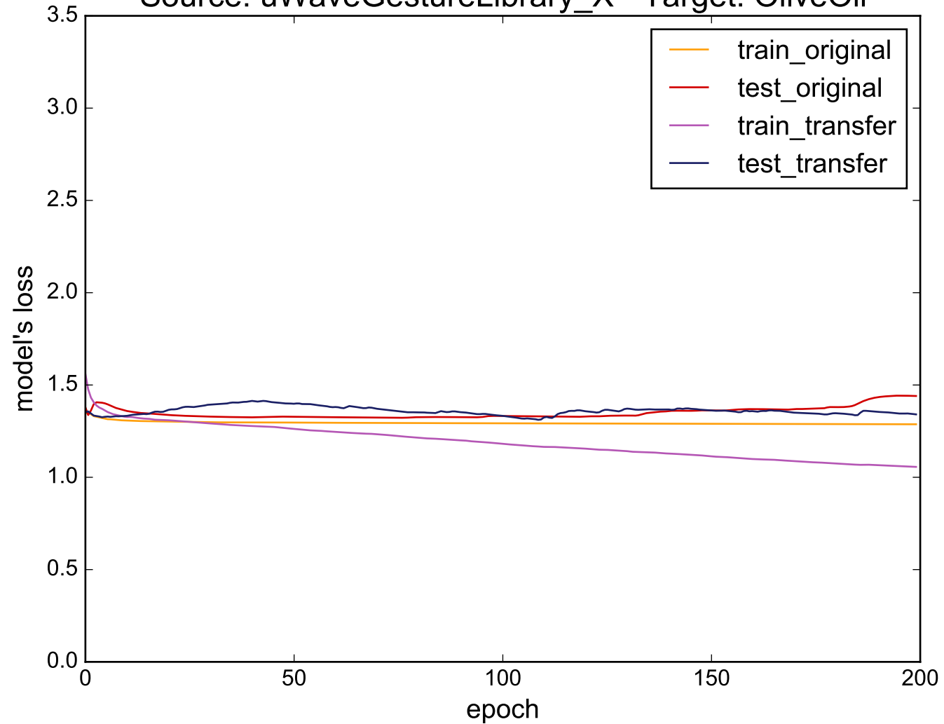
Source: uWaveGestureLibrary_X - Target: OliveOil
