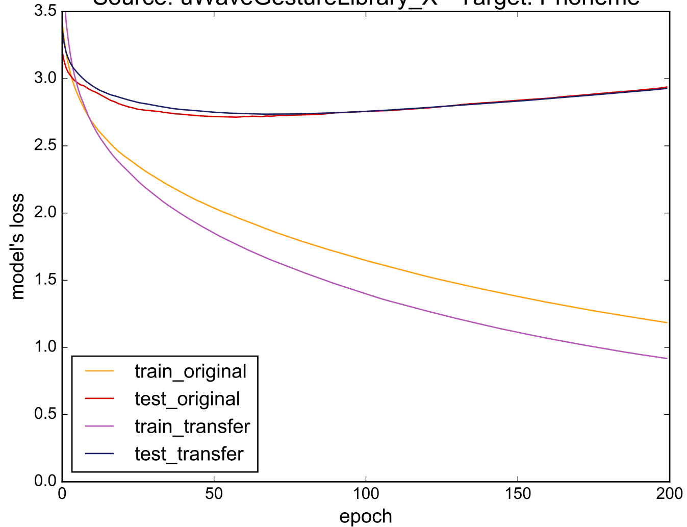
Source: uWaveGestureLibrary_X - Target: Phoneme
