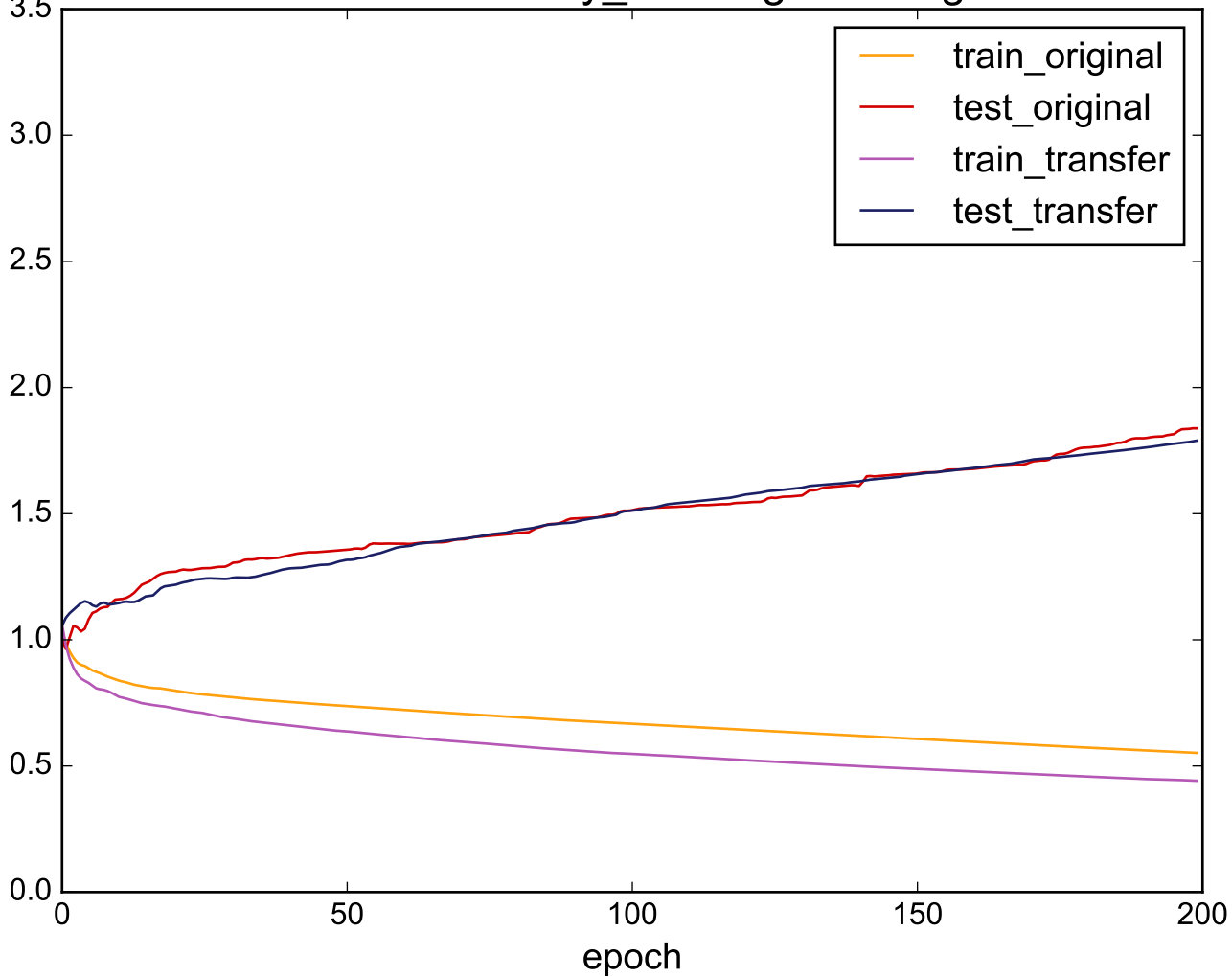
Source: uWaveGestureLibrary_X - Target: RefrigerationDevices
