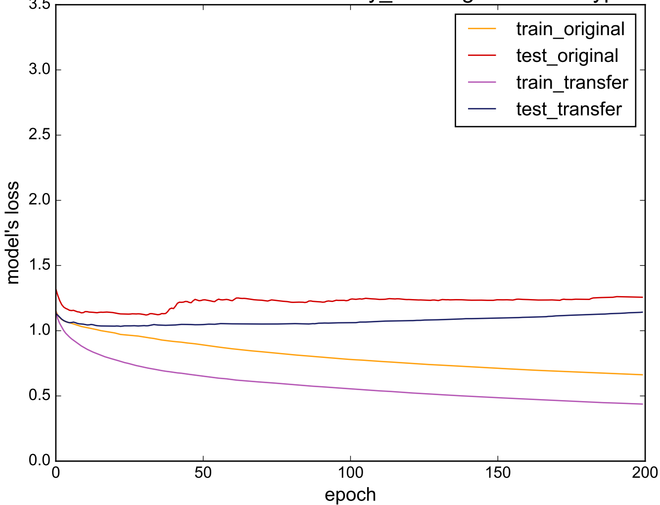
Source: uWaveGestureLibrary_X - Target: ScreenType
