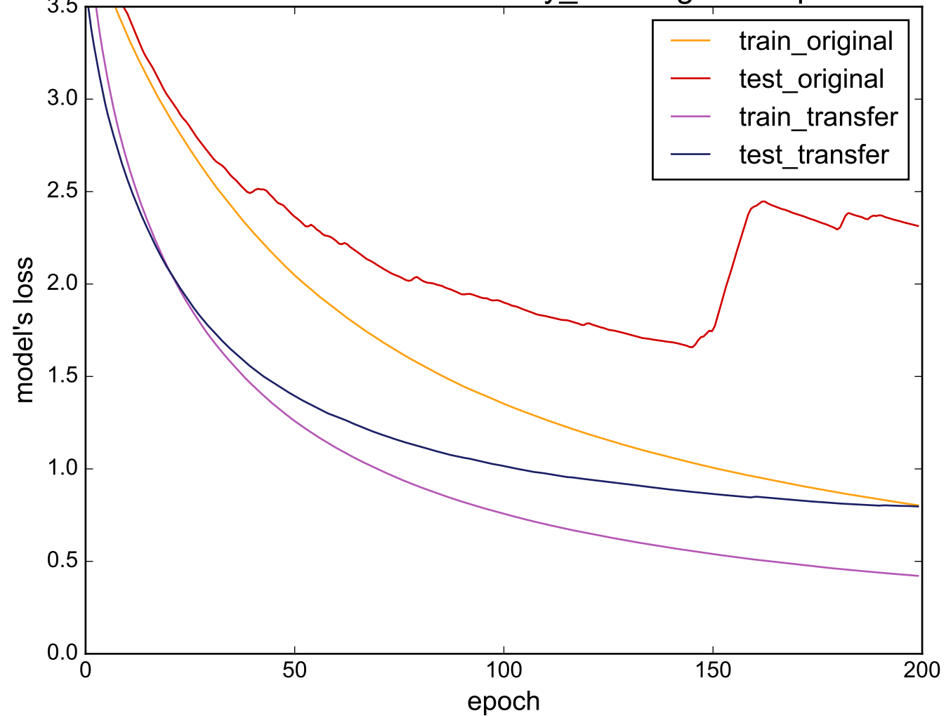
Source: uWaveGestureLibrary_X - Target: ShapesAll
