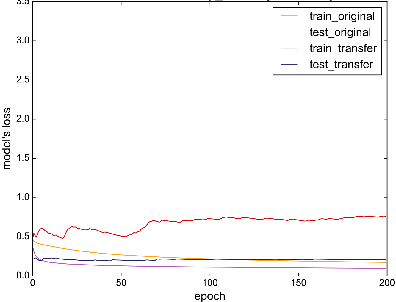
Source: uWaveGestureLibrary_X - Target: StarLightCurves
