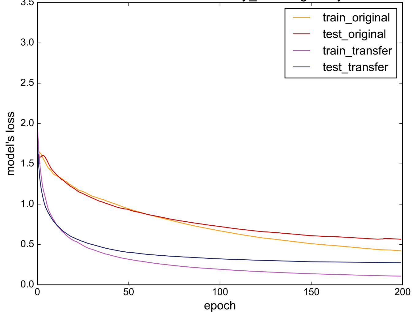
Source: uWaveGestureLibrary_X - Target: Symbols
