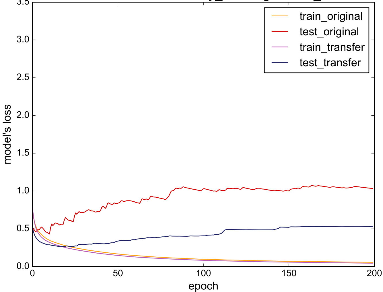
Source: uWaveGestureLibrary_X - Target: Two_Patterns
