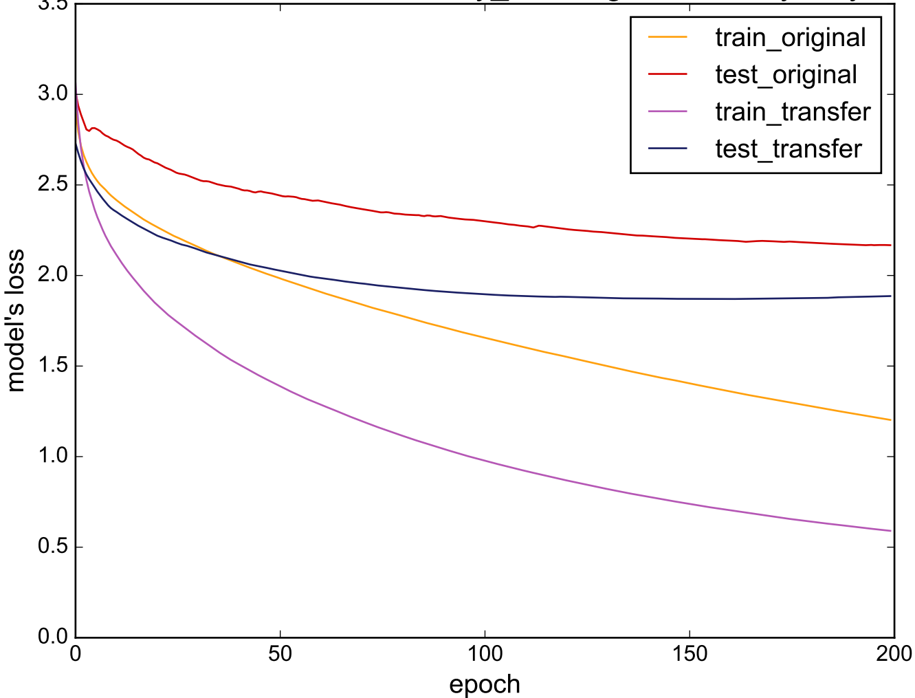
Source: uWaveGestureLibrary_X - Target: WordsSynonyms
