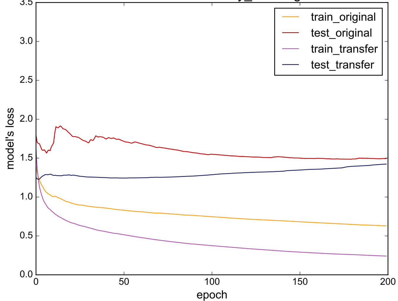
Source: uWaveGestureLibrary_X - Target: Worms
