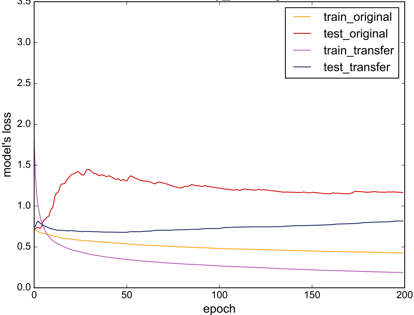
Source: uWaveGestureLibrary_X - Target: WormsTwoClass
