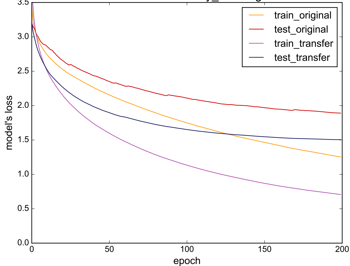
Source: uWaveGestureLibrary_Y - Target: 50words
