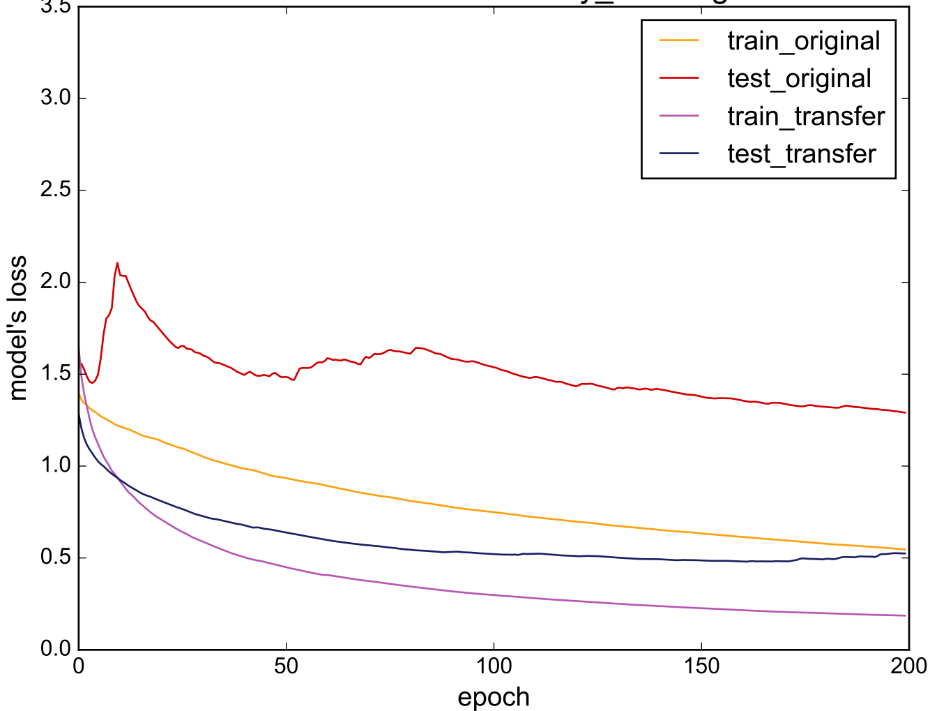
Source: uWaveGestureLibrary_Y - Target: Car
